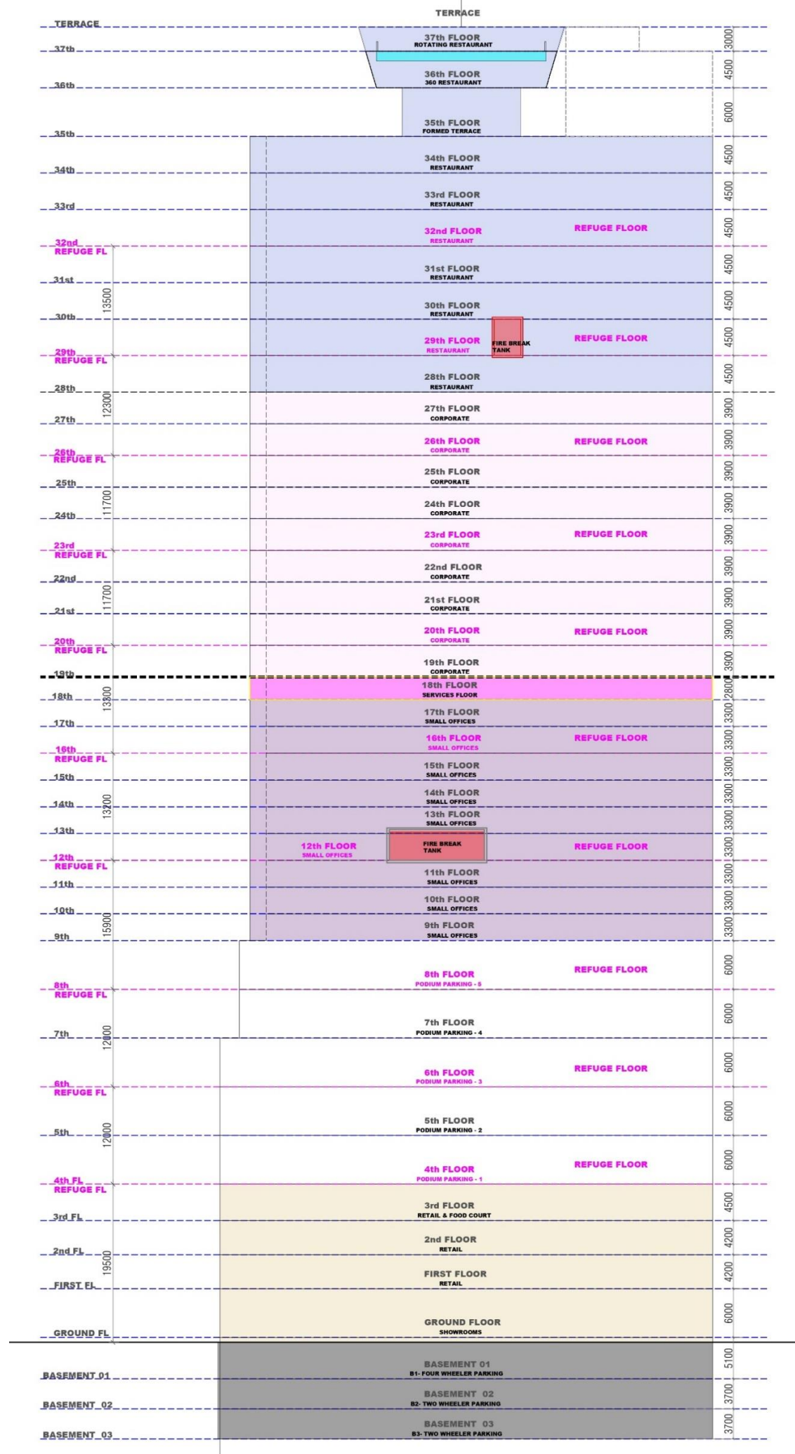
SCHMATIC SECTION
